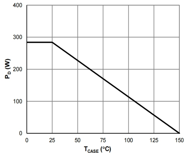
Figure 10: Power De-rating
