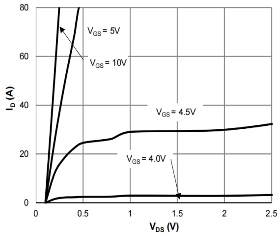
Figure 1: Saturation Characteristics
