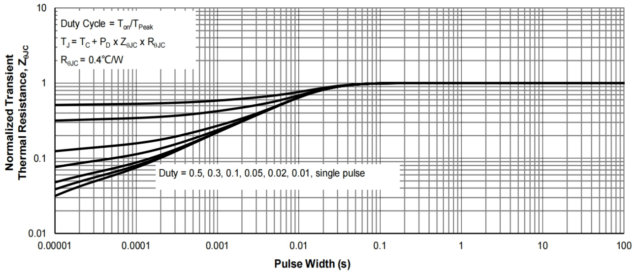
Figure 13: Normalized Transient Thermal Impedance
