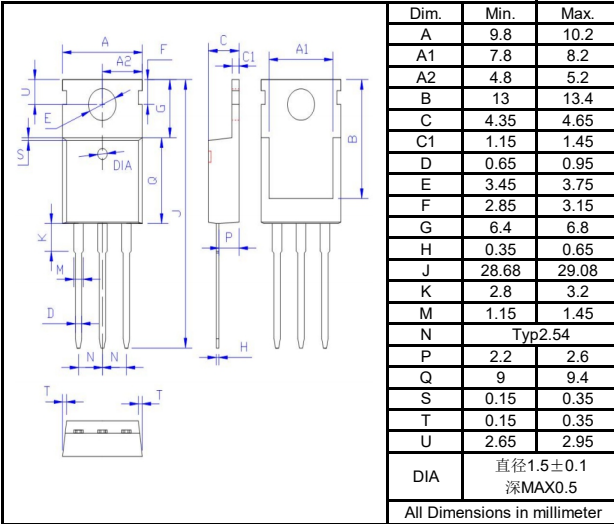
TO-220C
