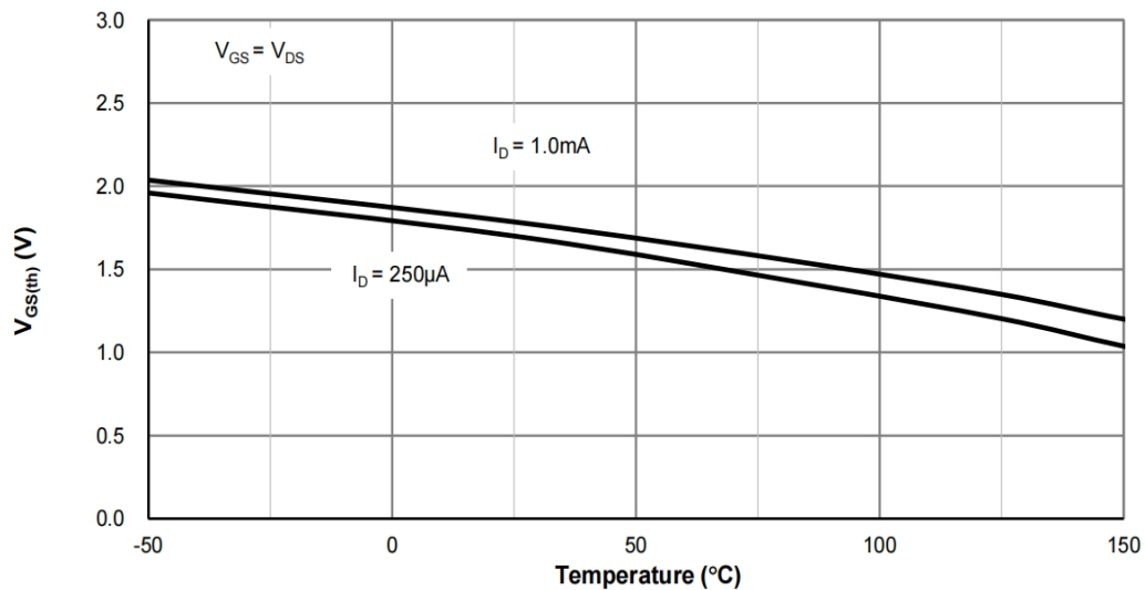
Figure 5: V_{GS(th)} vs. Junction Temperature
